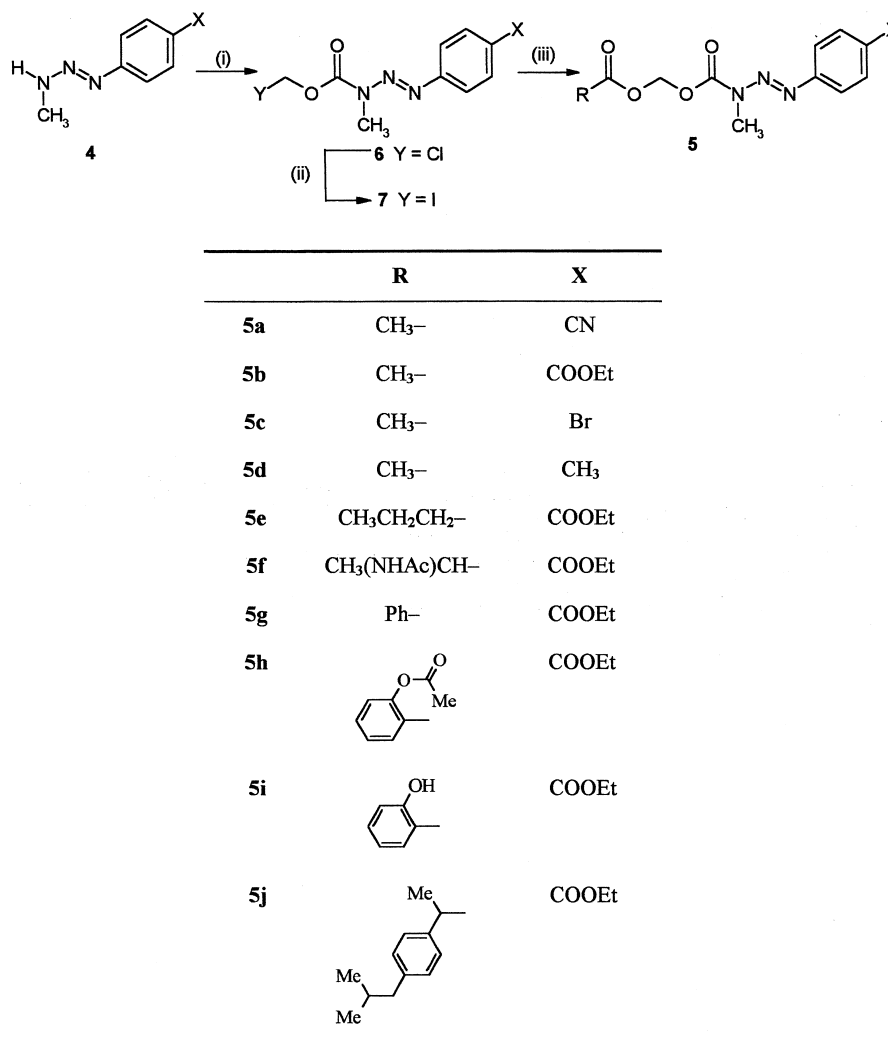
Figure 3. Synthesis and structures of the triazenes 5 . Reagents: (i) \text{ClCH}_2\text{OCOCl} ; (ii) \text{NaI} ; (iii) \text{RCO}_2\text{Ag} or \text{RCO}_2\text{H}/\text{Ag}_2\text{CO}_3 .
