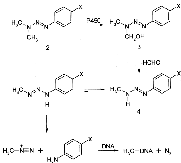
Figure 2. Oxidative demethylation pathway for 1-aryl-3,3-dimethyl-triazenes.
