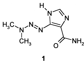
Figure 1. Structure of dacarbazine.
