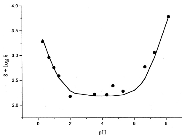
Figure 4. pH–Rate profile for the hydrolysis of 5f ; points are experimental, line is best fit using rate constants for the acid-, base- and uncatalysed hydrolyses of 4 \times 10^{-5} \text{ M}^{-1} \text{ s}^{-1} , 42.3 \text{ M}^{-1} \text{ s}^{-1} and 1.55 \times 10^{-6} \text{ s}^{-1} , respectively.
