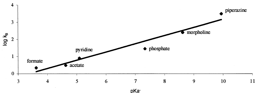
Figure 5. Brønsted plot for the buffer-catalysed hydrolysis of 5f .
