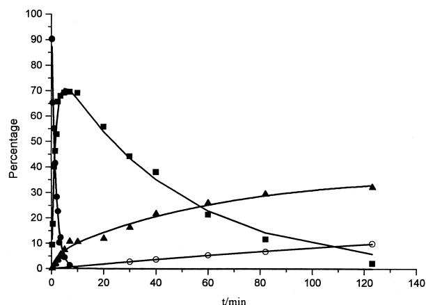
Figure 6. Time course for the formation and decay of intermediates in the plasma mediated cleavage of 5h : ●, 5h ; ■, 5i ; ▲, 4 ; ○, aniline (X = COOEt).
